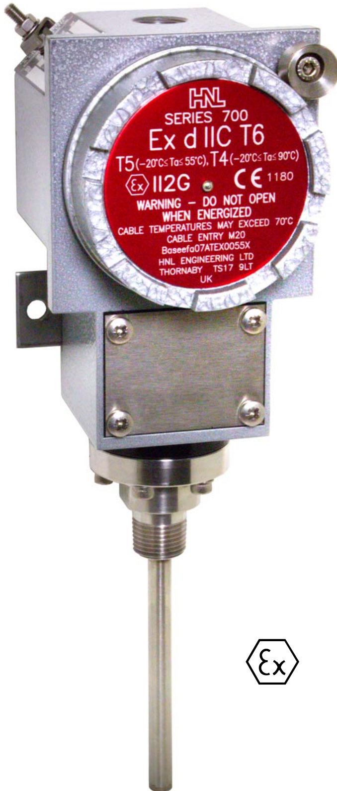
DIRECT MOUNTING VERSION SHOWN – ALSO AVAILABLE WITH CAPILLARY
